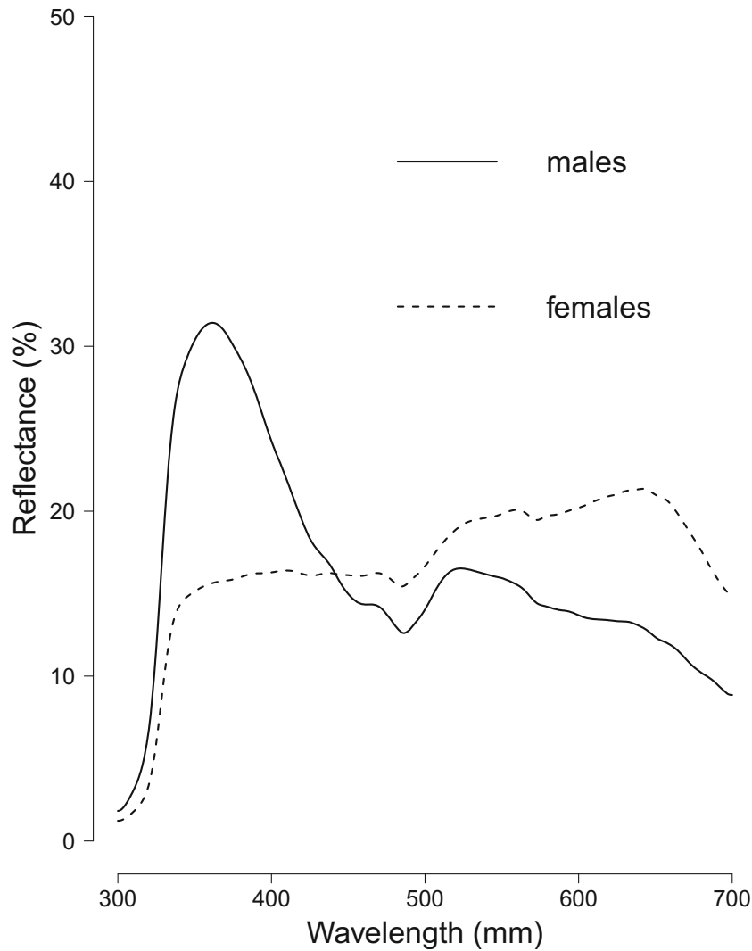
Fig. 1 Mean reflectance spectra and 95% confidence interval curves of UV-blue spots for males and females. The male mean spectrum distinctly peaks in reflectance in the UV region ( \lambda_{max} = 360–365 nm) while the
