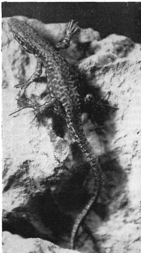
Lacerta muralis
